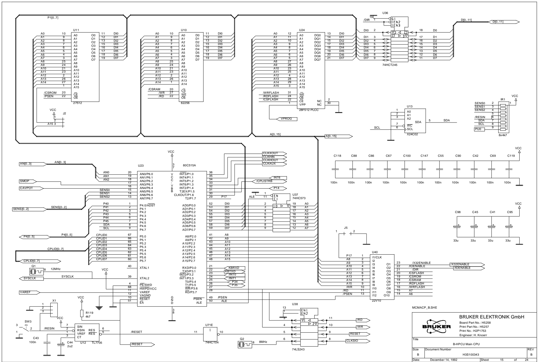
Figure 12.15.B-HPCPU Main CPU
