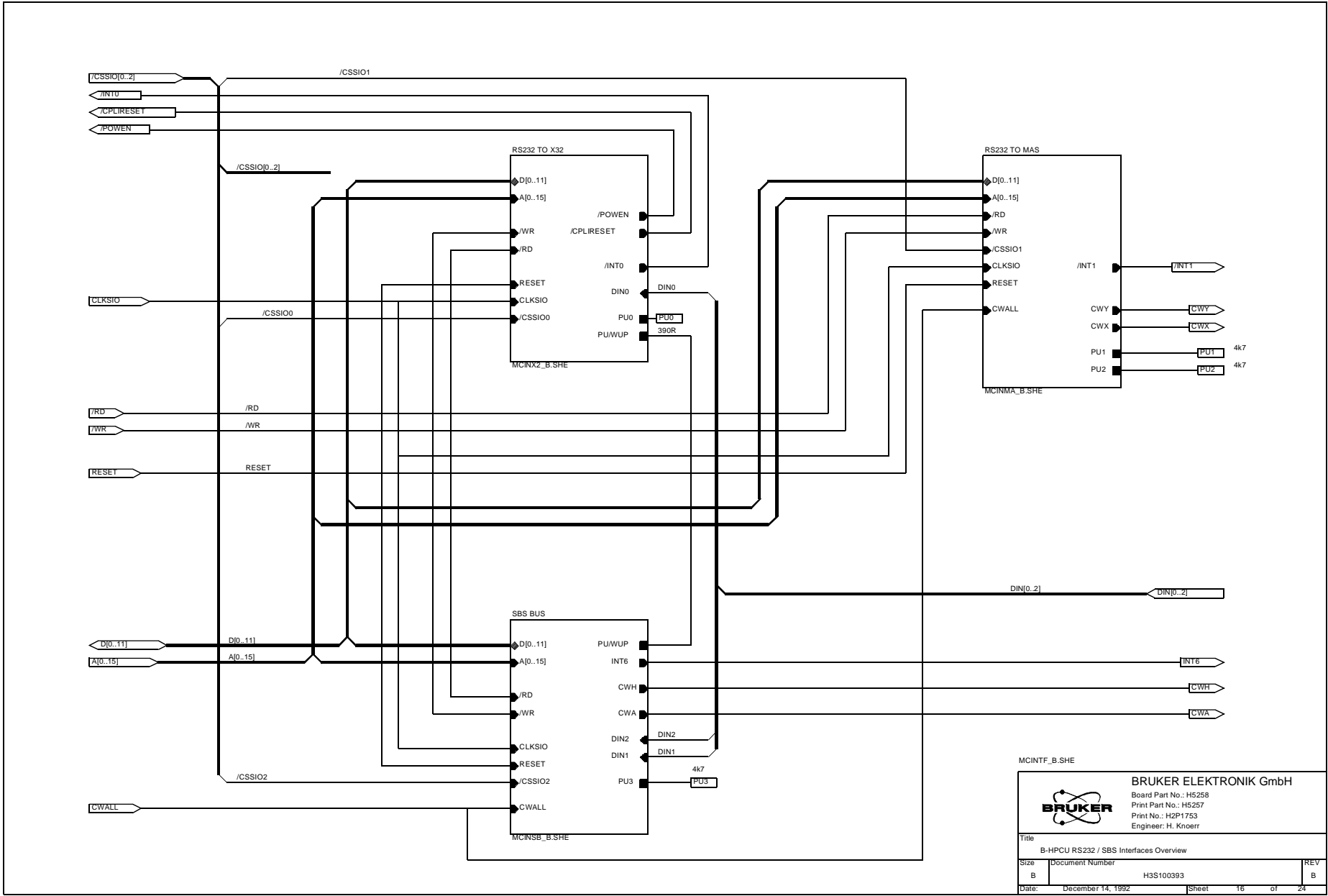
Figure 12.16: B-HPCU RS232/SBS Interface Overview
